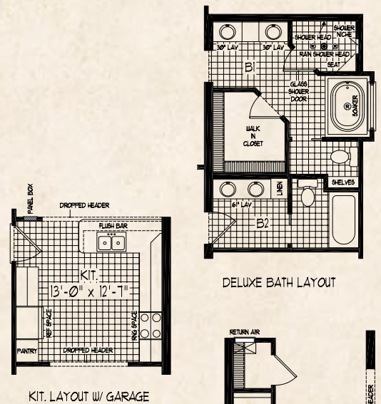
KIT. LAYOUT W/ GARAGE
